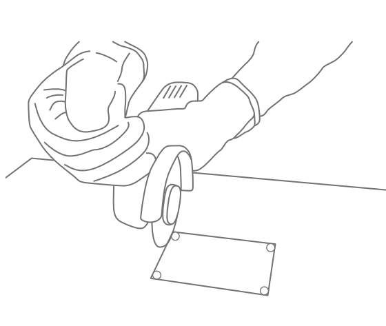
For L-shaped cuts or cuts inside the slab, holes should be bored at the vertices to prevent the blade of the cutting disk damaging the surface.
