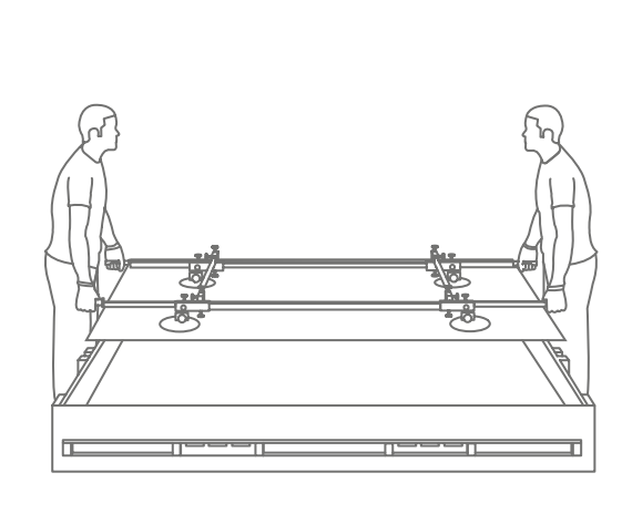
Handling the slabs on the floor can be managed with the aid of a frame fitted with suction cups to make the slabs more stable.
