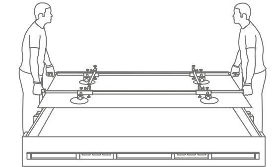
Handling the slabs on the floor can be managed with the aid of a frame fitted with suction cups to make the slabs more stable.
